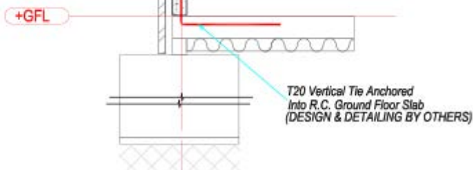
Typical Detail of Reinforcement for Ground Floor and Upper Levels
